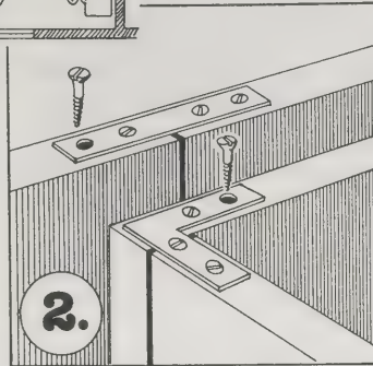
Doors are fastened, top and bottom, with metal "corner irons" and wood screws (Illustration 2).
